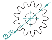
Cogwheel 13 teeth (Z)
